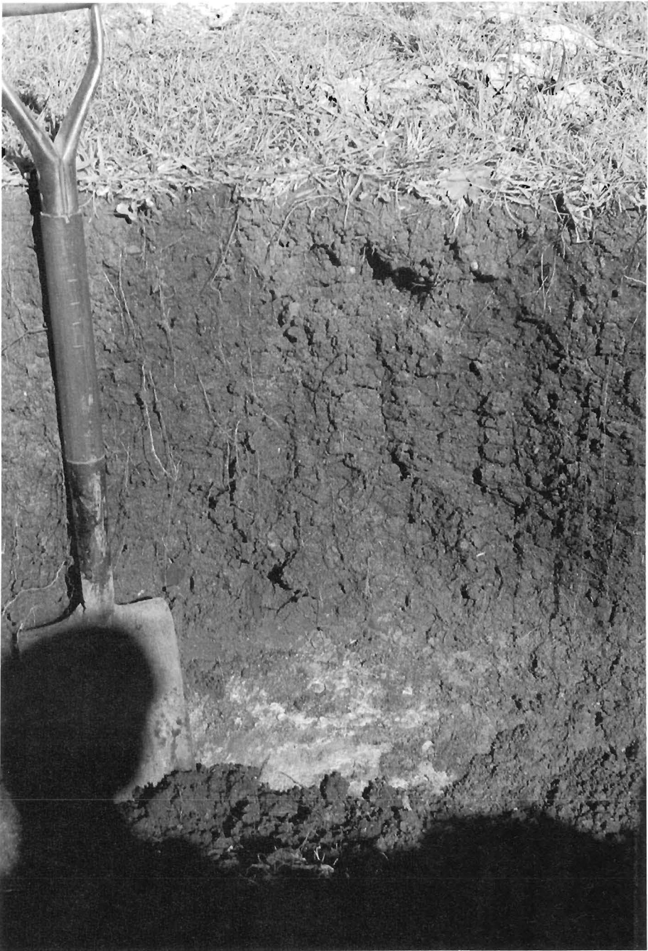
FIG. 2.—Weakly developed soil with some horizonation. Mollic epipedon in A; Argillic in B.
