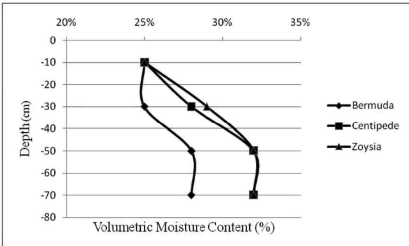
FIGURE 4. Soil moisture content in relation to the depth and grass type, corresponding to the level of 125% ET on 11 June 2002.
