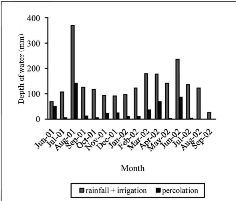
FIGURE 5. Monthly precipitation and irrigation and the average percolation from all the treatments.
